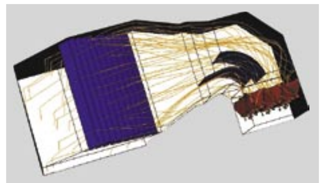
Streak lines of ammonia injected in front of a SMV Mixer with extremely limited space available in front of the catalyst
