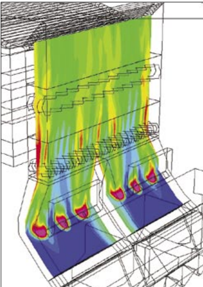
Temperature homogenization upstream of a flue gas heater
