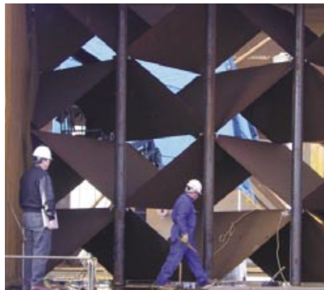
Inspection on an SMV Mixer with Sulzer Ammonia Injector
