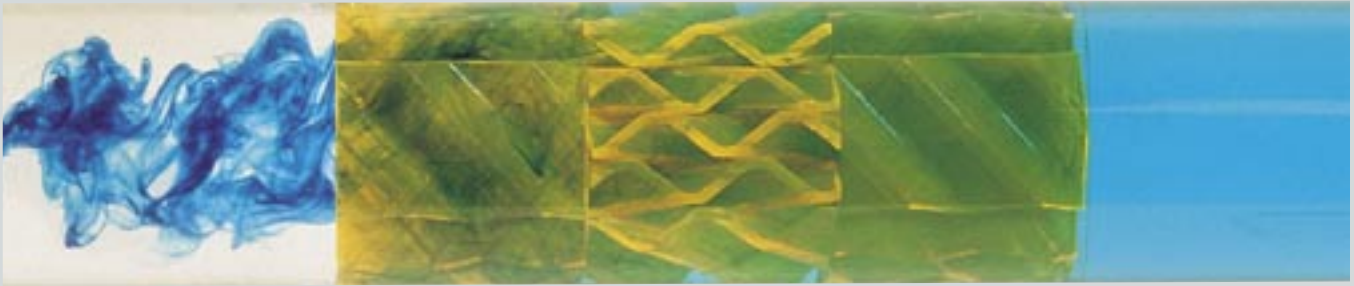
Sulzer SMV Mixer for continuous in line mixing of additives. As shown, the mixer length required for a high degree of homogeneity is short.
